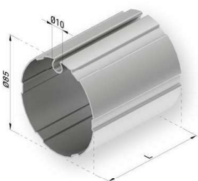
Barra de enrollle Ø85
